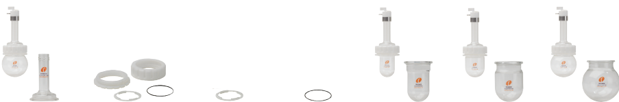
RR99946 Wide Neck Reflux Tube + Coupling RR99925 Coupling for Wide Neck Flasks RR99940 PTFE Wide Neck Support Collar RR99941 Nitrile O-Ring for PTFE Wide Neck Flask RR99926 50ml Wide Neck Flask RR99928 100ml Wide Neck Flask RR99933 250ml Wide Neck Flask
